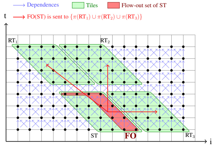
Figure 6.2: FO scheme for stencil
