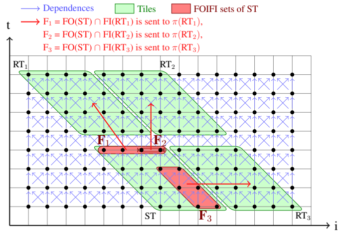
Figure 6.3: FOIFI scheme for stencil
